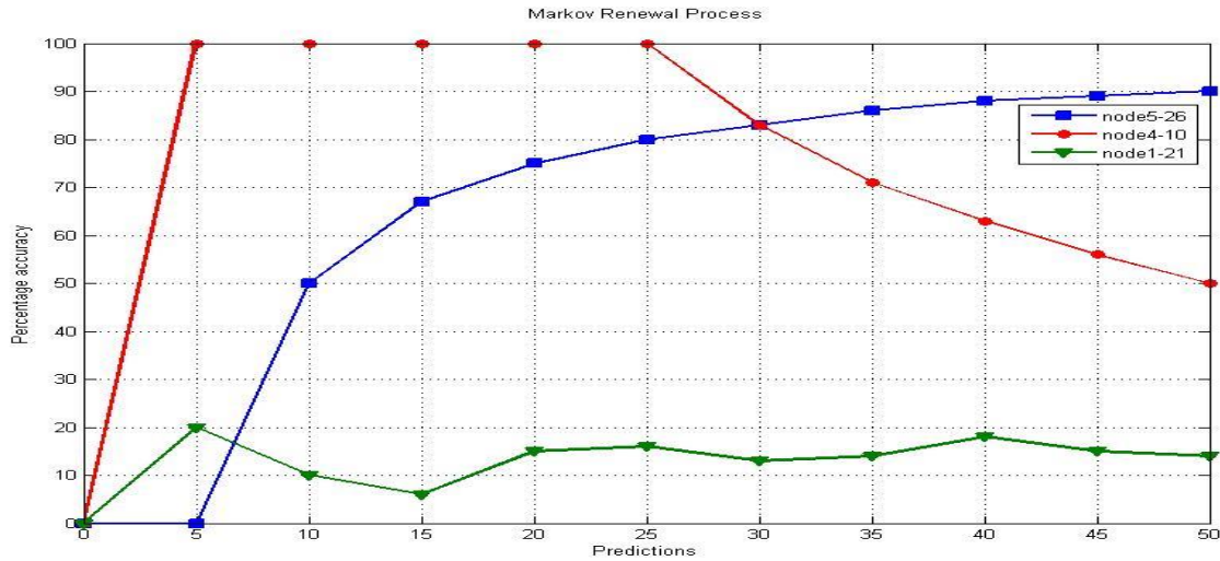
Figure 6: Markov Chains average prediction accuracy
