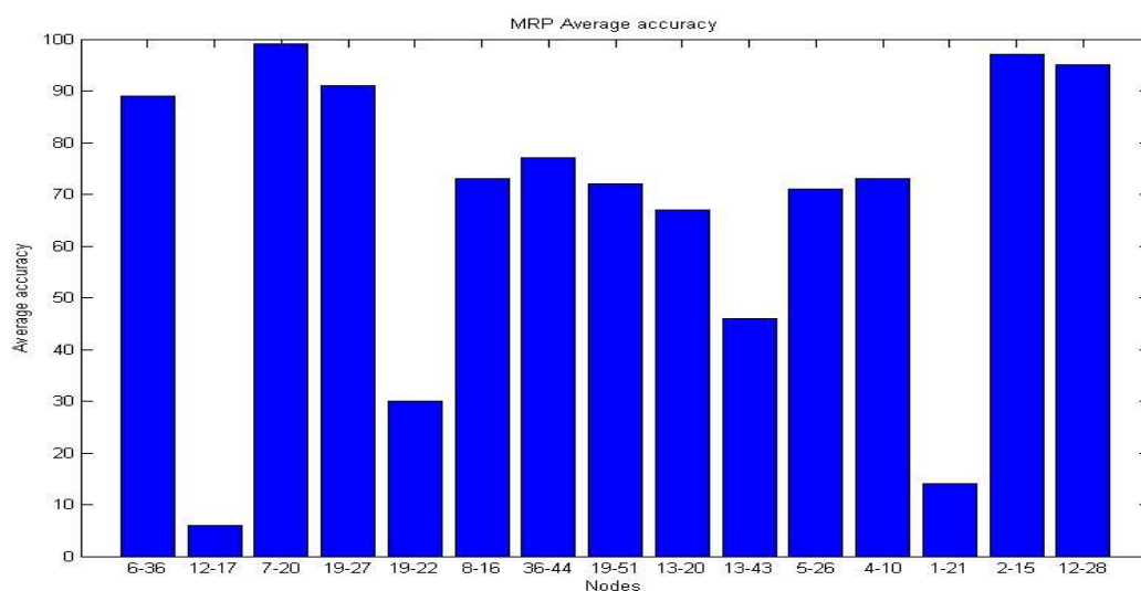
Figure 7: MRP average prediction accuracy
