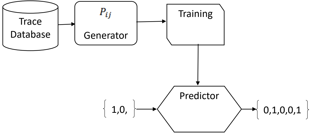
Figure 1: Markov chain prediction model
